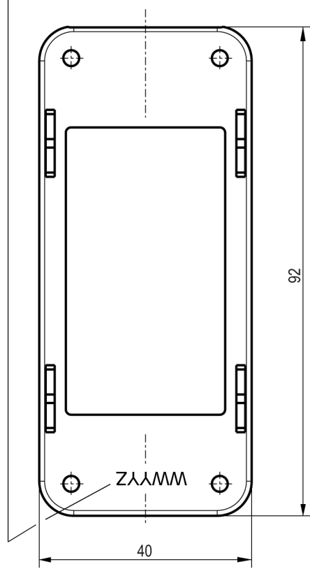
Schriftfelder vertieft / Inscription fields deepened
